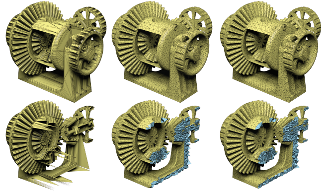
Fig. 9. Voxel stuffing produces a tetrahedral mesh (middle) of quality comparable to a direct BSP-tree construction (right), but reduces the running times from 3292.3 seconds to 2476.6 seconds.
