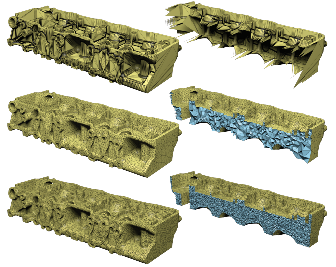
Fig. 17. \ell controls the density of the output mesh. Input (top), \ell = b/20 (middle) and \ell = b/150 (bottom).
