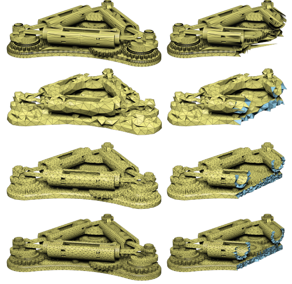
Fig. 4. An oversized \epsilon ( \frac{b}{100} , with b being the bounding box diagonal) creates a tetrahedral mesh (2nd row) that fails to capture the features of the input triangle mesh (1st row). Reducing \epsilon to \frac{b}{300} and \frac{b}{3000} increases the geometric fidelity (3rd and 4th row).
