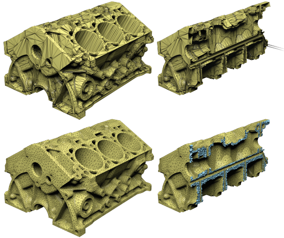
Fig. 6. A low quality triangle mesh exported from a CAD model with Open-Cascade (top) is automatically converted into a high-quality tetrahedral mesh by our algorithm (bottom), without requiring any manual cleanup.
