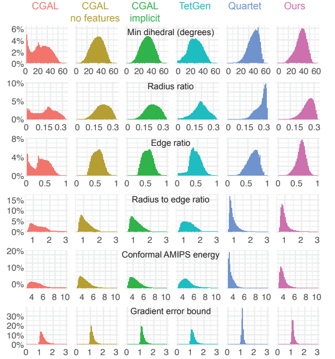
Fig. 14. Comparison of generated mesh quality on Thingi10k dataset. For each software, we show the distribution of 6 common quality measures of all tetrahedra in 1000 randomly sampled meshes generated from Thingi10k dataset. Quality measures: dihedral angle, inscribed/circumscribed sphere radius ratio, conformal AMIPS energy, and normalized Shewchuk's gradient error estimate factor ([Shewchuk 2002b]).
